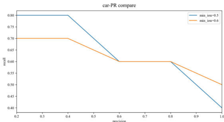
图 6-34 car-PR compare
